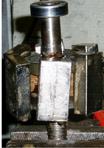
Figure 1. 40 Amp car alternator rotor with magnets attached
