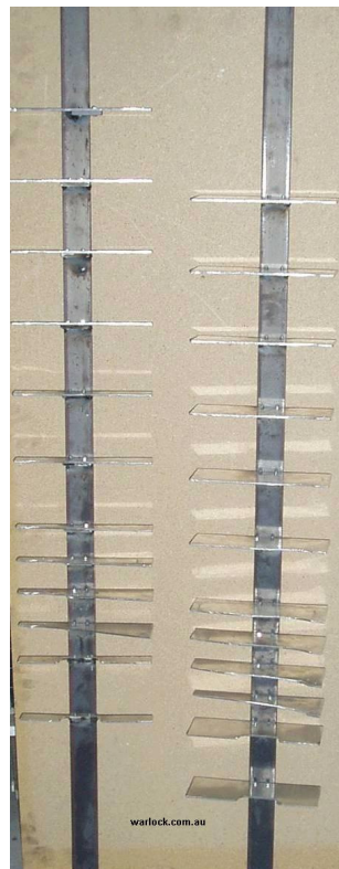
Figure 7. Wind turbine airfoil cross-sections bolted to frame
